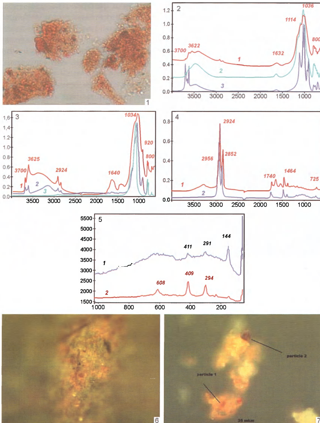
Fig. 3. Lanino 1/8, engraved pebble: 1 — particle from sample 2, microphotography in polarized light; 2–4 — infrared spectra (2: 1 — surface layer stone material; 2 — mixture of potassium-sodium feldspars and kaolinite, 3 — kaolinite; 3: 1 — outer layers of the sample 2; 2 — yellow ocher with an admixture of kaolinite and quartz; 3 — quartz; 4 — extracts in chloroform of sample 3 with differences in the molecular composition of its components: 1 — with the presence of substances of lipid and protein nature; 2 — with domination of substances of lipid nature); 5 — Raman spectra of the mineral inclusions in the paint layer of sample 2 (1 — yellow-red particles; 2 — dark red particles); 6, 7 — microphotographs in reflected light (6 — pebble surface, magnification 20×; 7 — outer [red] later of sample 3, magnification 50×)
